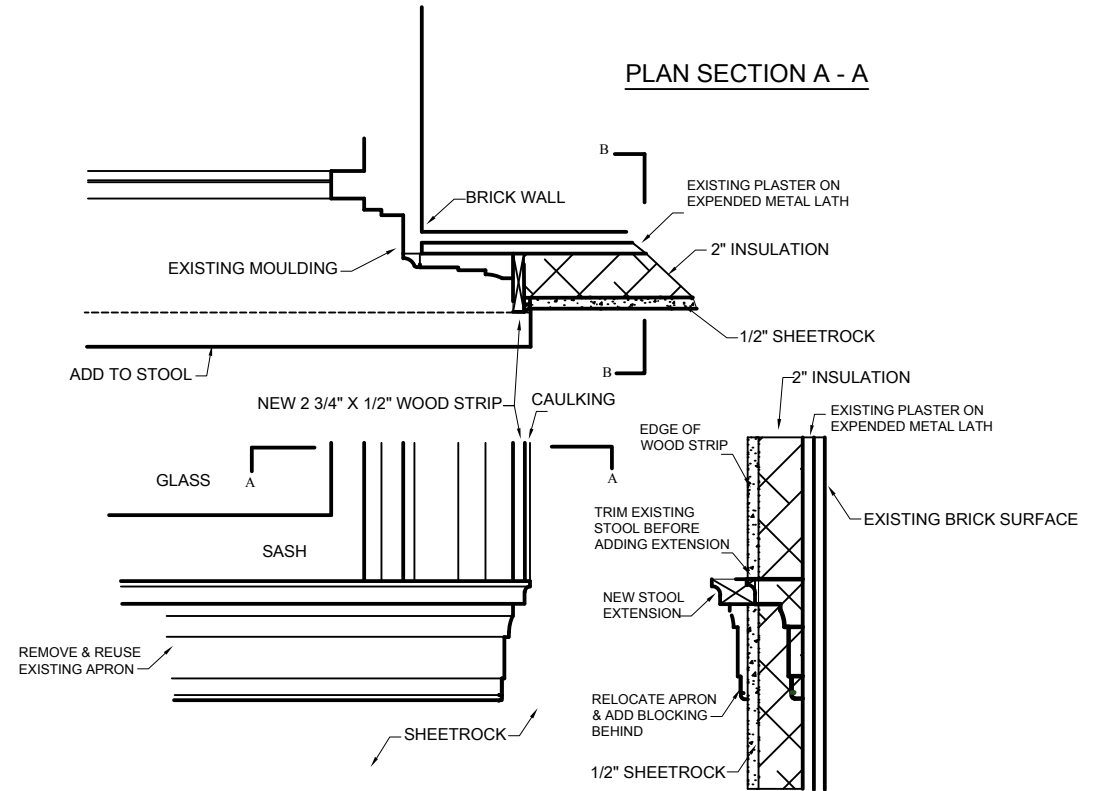
DETAIL ELEVATION
